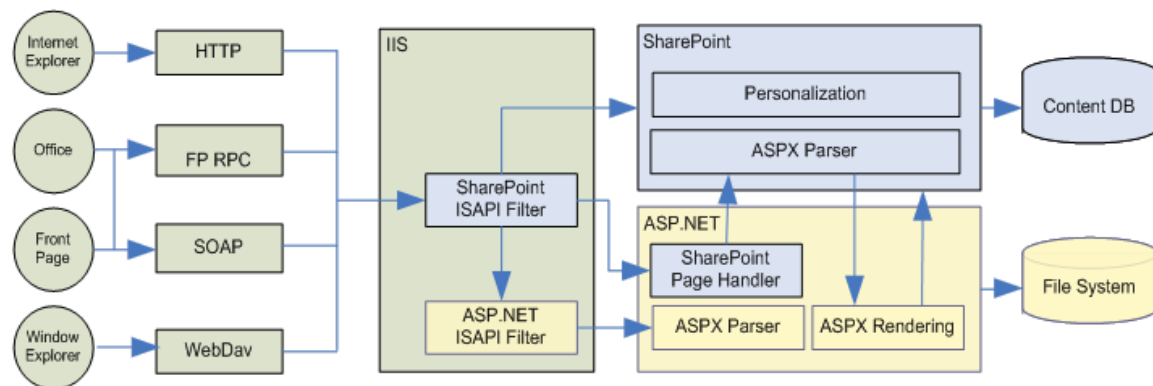
Figure 27. Windows SharePoint Services 2.0 SP2 architecture
